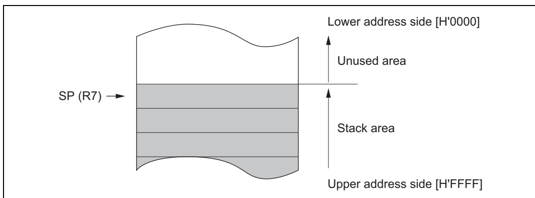
Figure 2.2 Stack Pointer
